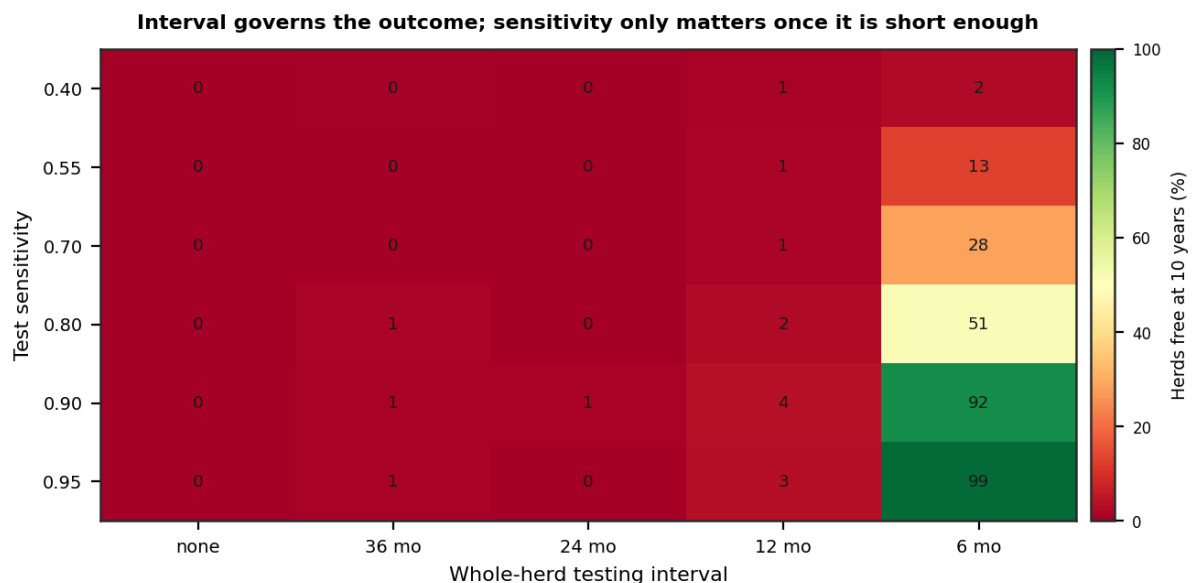
Figure 3. Herds free of infection at 10 years across sensitivity and testing interval.
