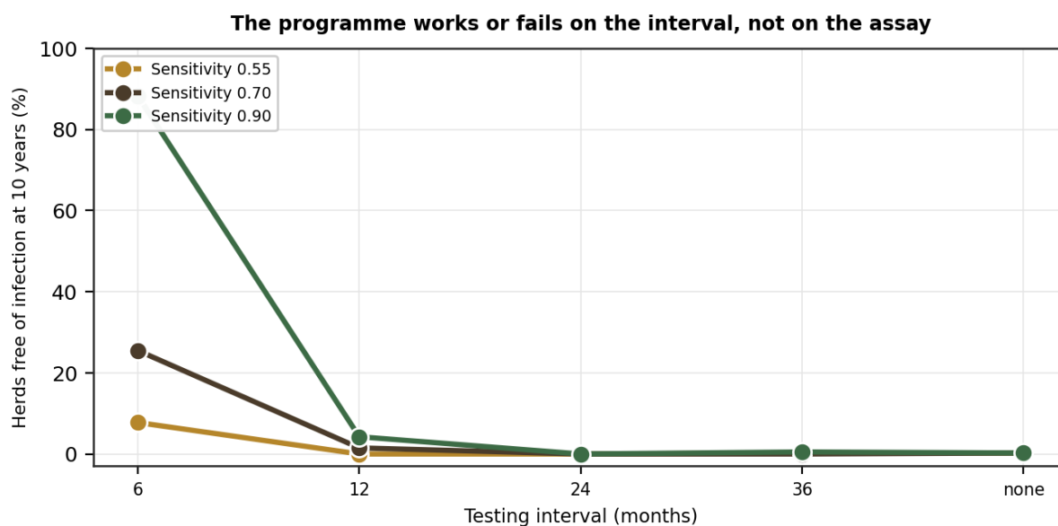
Figure 4. Herd freedom against testing interval at three levels of sensitivity.
