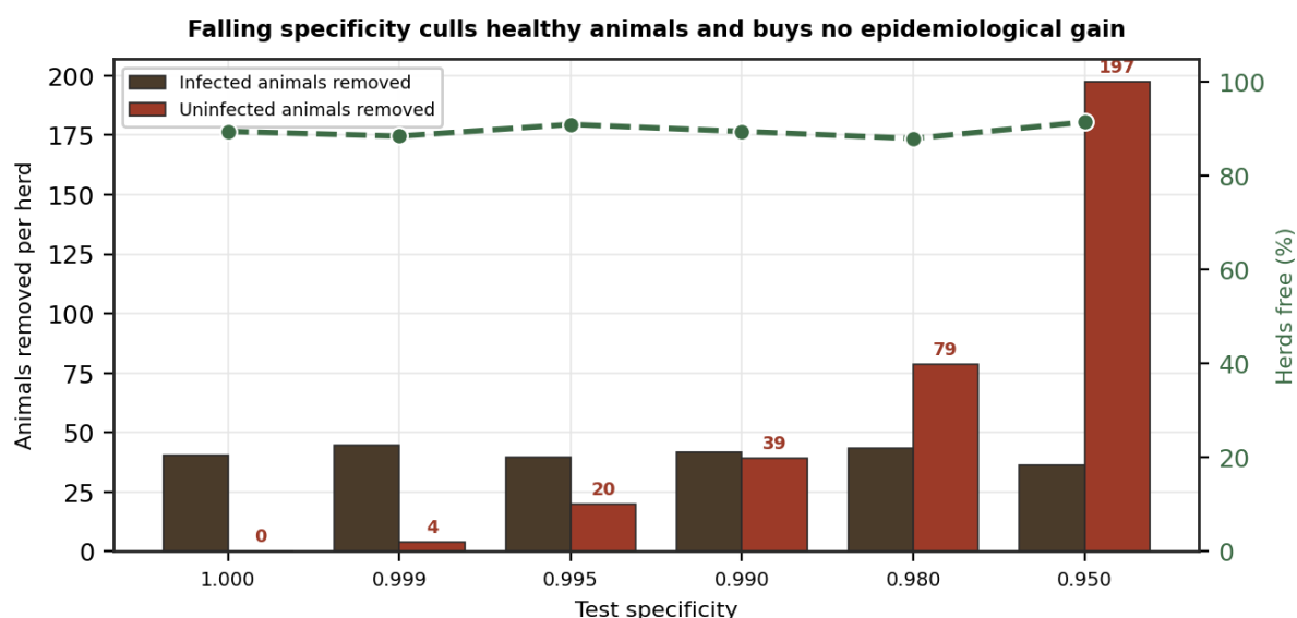
Figure 5. Animals removed and herd freedom against test specificity.
