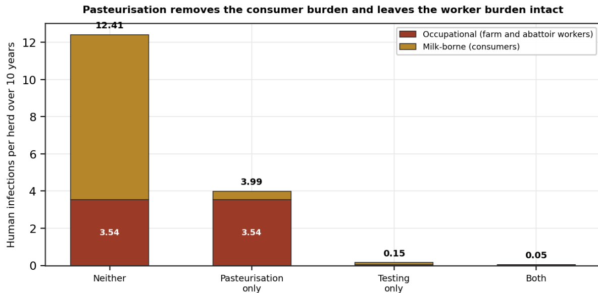
Figure 6. Human infections by pathway under testing, pasteurisation, both and neither.
