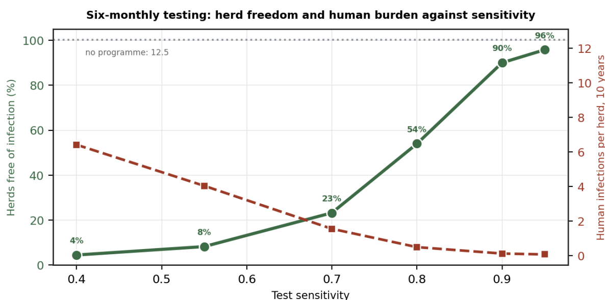
Figure 2. Herd freedom and human infection against test sensitivity under 6-monthly testing.
