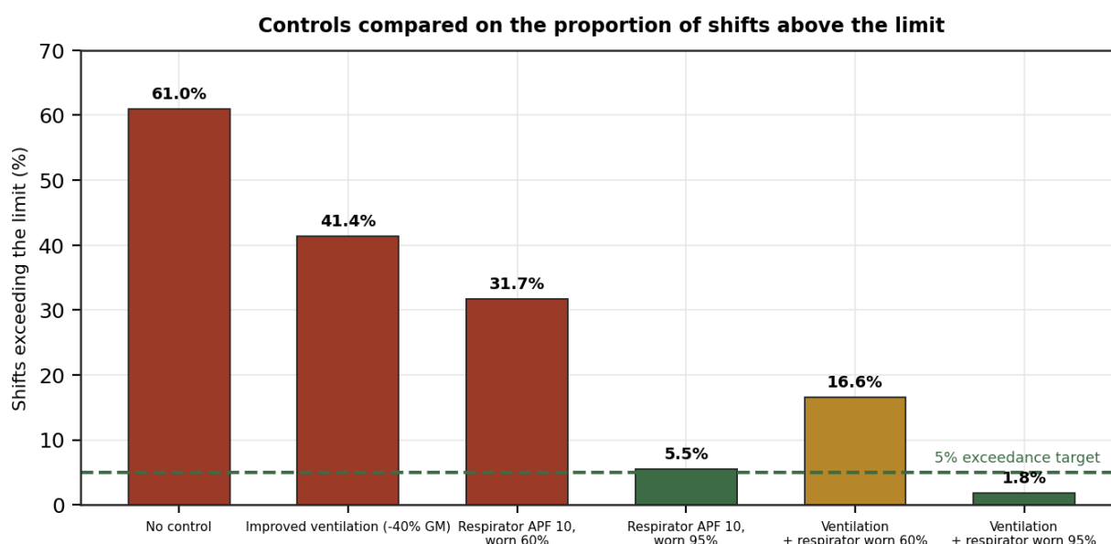
Figure 5. Proportion of shifts above the limit under six control configurations.
