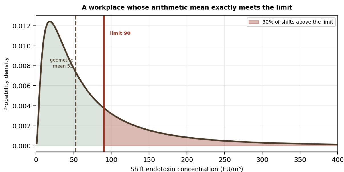
Figure 1. Shift exposure distribution for a workplace whose arithmetic mean sits exactly at the limit.
