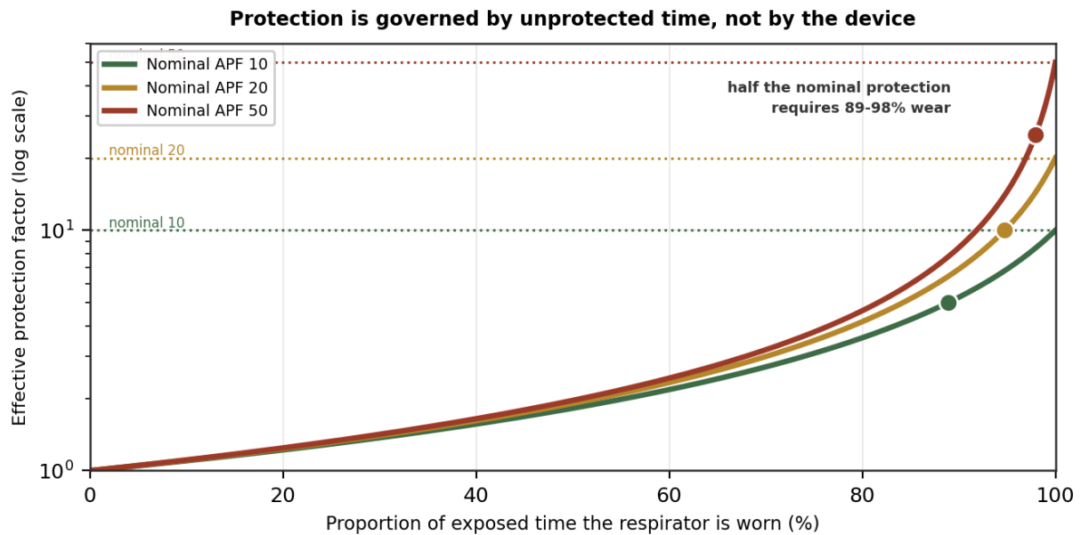
Figure 4. Effective protection factor against the proportion of exposed time the respirator is worn.
